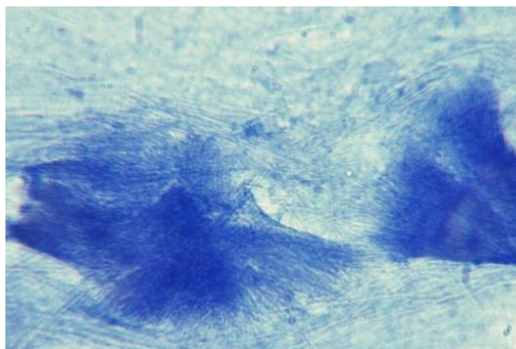
Fig. 2: Amorphous granular material (Pap 40x) (Inset showing elongated crystals)
