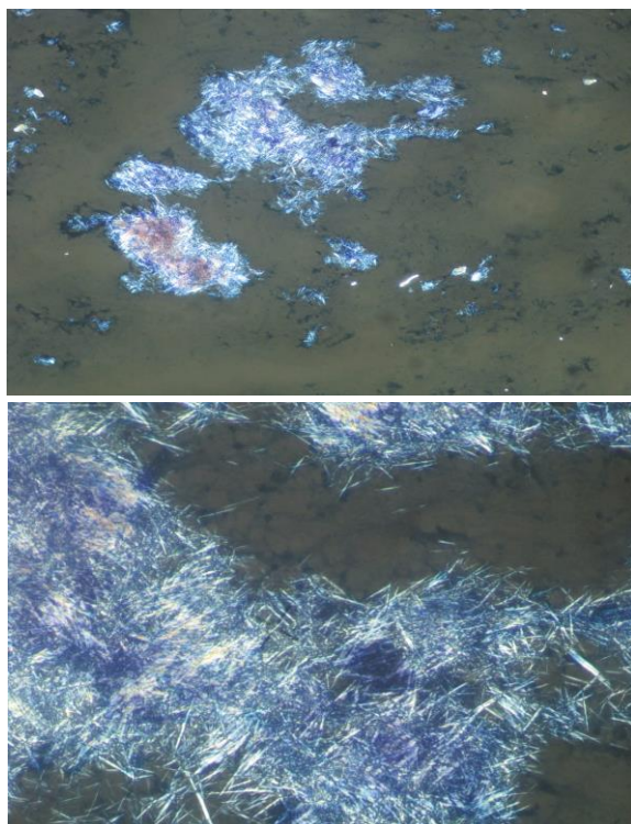
Fig. 3: Elongated needle shaped crystals under polarising light (Pap stain 40x)
