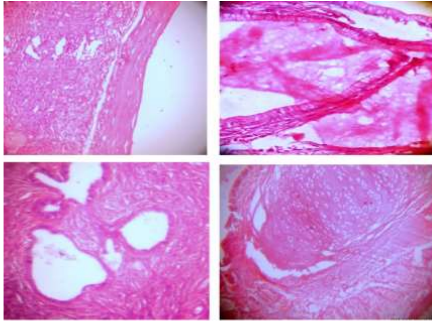
Fig. 3: Photomicrograph showing histopathological features of benign neoplastic ovarian lesions: a) Serous cyst adenoma b) Mucinous cyst adenoma(tall coloumnar cell lining and mucin) c) Endometrioid tumor (endometrial gland in ovarian stroma) d) Benign cystic teratoma (Cartilage, Squamous cell lining, sebaceous gland)
