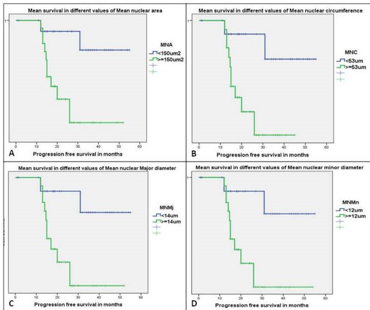
Fig. 2: Kaplan meier plots of the probability of progression-free survival (PFS) in patients with RCC. A: Mean PFS for tumors with MNA \geq 150\mu\text{m}^2 vs MNA <150\mu\text{m}^2 , B: Mean PFS for tumors with MNC \geq 53\mu\text{m} vs MNC <53\mu\text{m} , C: Mean PFS for tumors with MNMj \geq 14\mu\text{m} vs MNMj <14\mu\text{m} , D: Mean PFS for tumors with MNMn \geq 12\mu\text{m} vs MNMn <12\mu\text{m}
